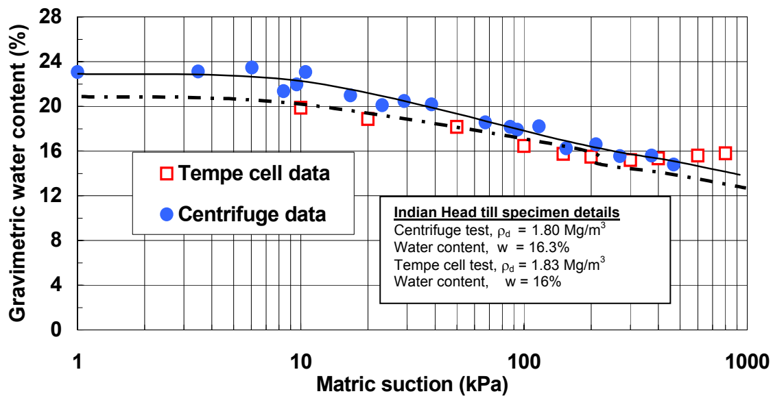
Figure 8. Comparison of measured soil-water characteristic curve using Tempe cell and centrifuge method for Indian Head Till specimens with initial water content of 16.3%.
